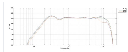
Direct Sound Frequency Response
