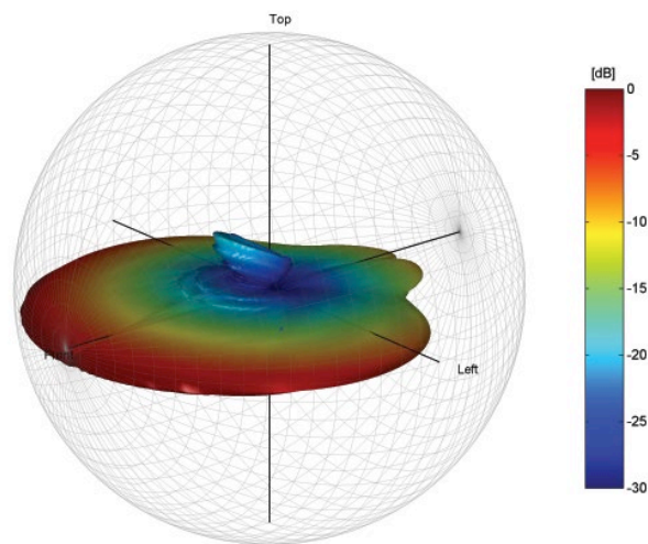
Intellivox DDC 3D directivity balloon
